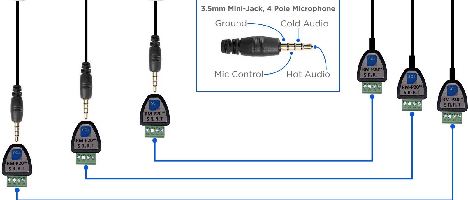
Female TRRS to 4pin Phoenix
