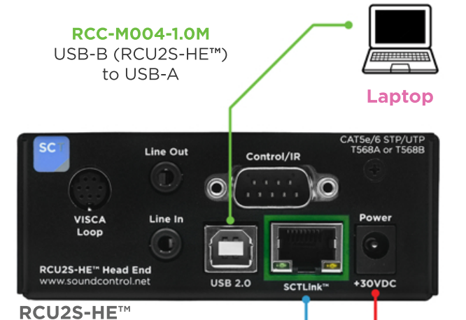
RCU2S-HE™ Front Panel Field-Upgradeable microSD Slot
